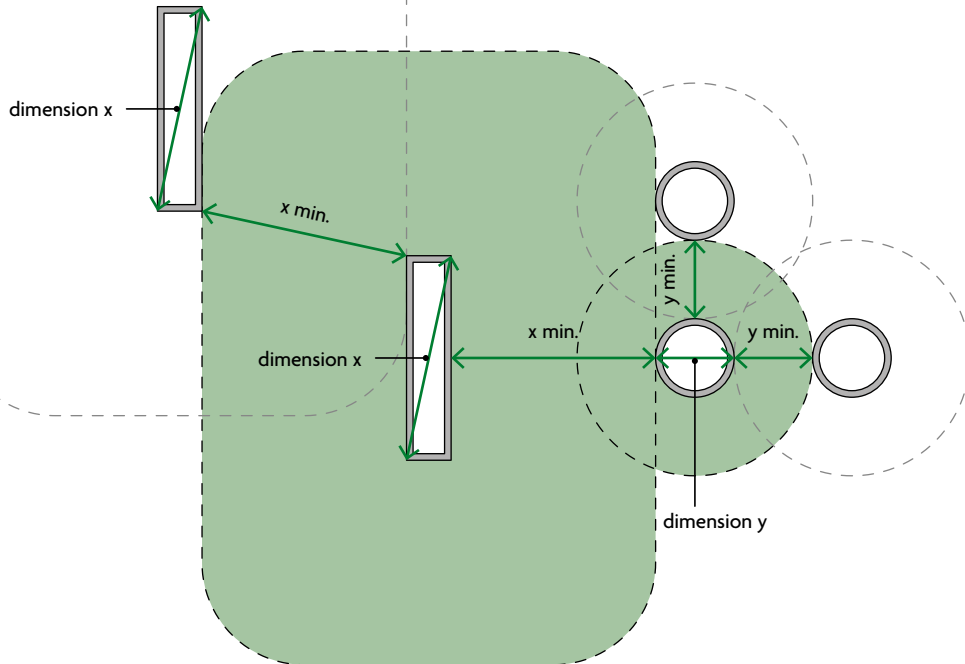
Ceiling plan
