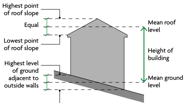
a. Double pitch roof
