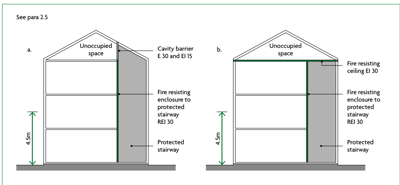
Diagram 2.3 Alternative cavity barrier arrangements in roof space over protected stairway in a house with a storey more than 4.5m above ground level
