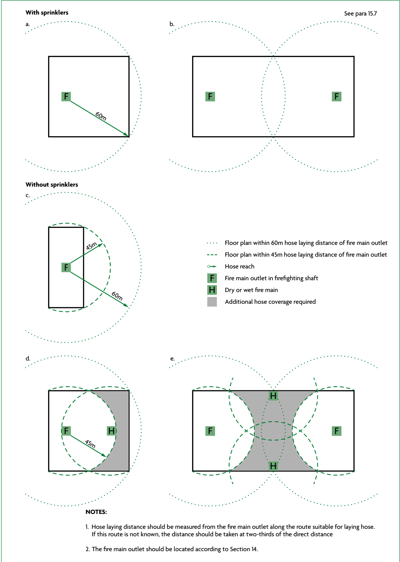
Diagram 15.3 Location of firefighting shafts: hose laying distances
