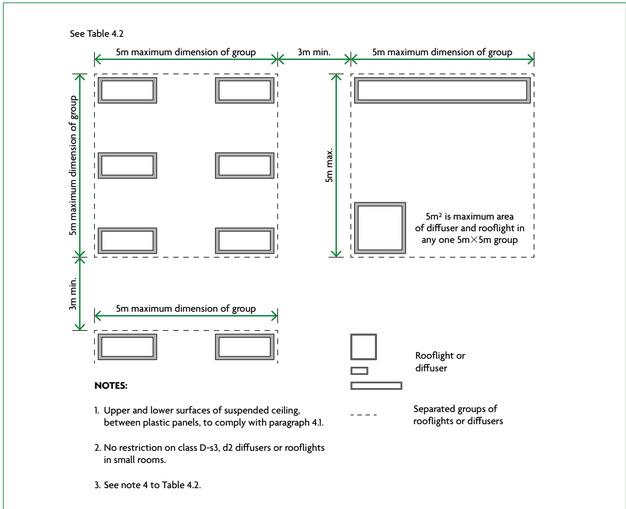
Diagram 4.2 Layout restrictions on class D-s3, d2 plastic rooflights, TP(b) rooflights and TP(b) lighting diffusers
