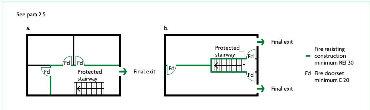
Diagram 2.2 Alternative arrangements for final exits
