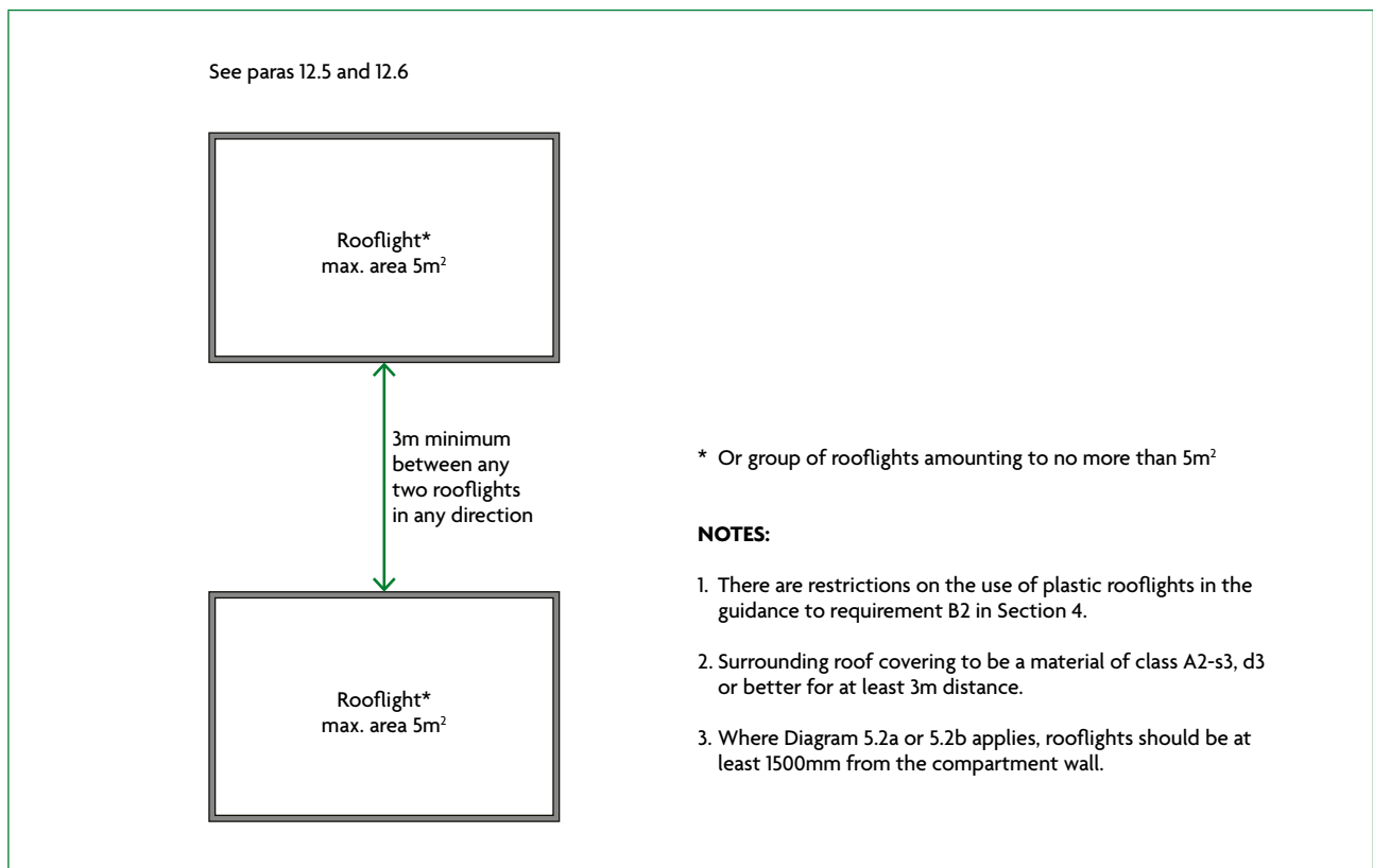
Diagram 12.1 Limitations on spacing and size of plastic rooflights that have a class D-s3, d2 or TP(b) lower surface
