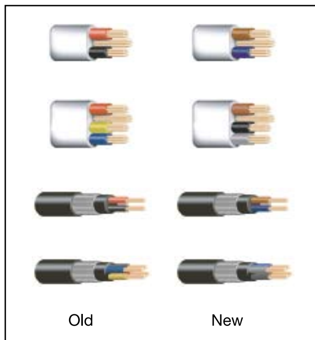
Diagram D1 Examples of cable with old and new colours
