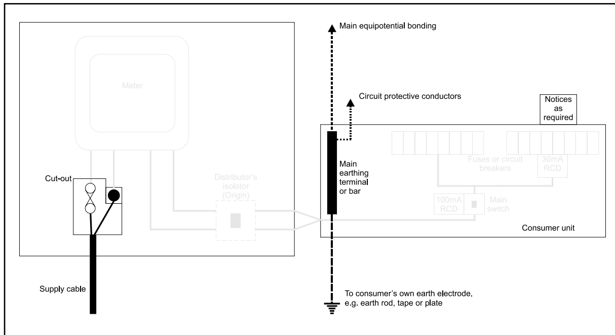
Diagram 2(b) Example earthing arrangement where consumers provide their own earthing connection (referred to as a TT system).
